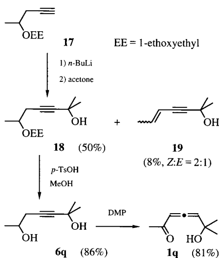
Scheme 5
